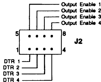
Figure 20: Half Duplex Jumper Configuration
