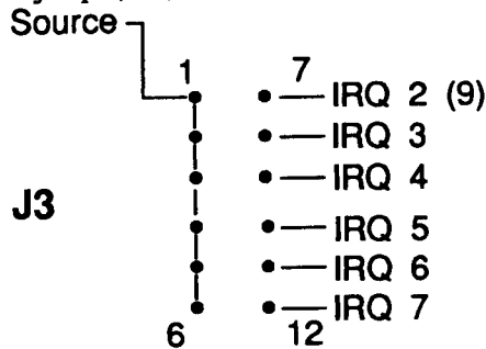
Figure 17: Interrupt Level Selection Jumper
