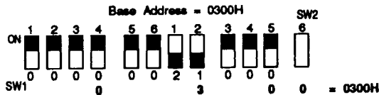
Figure 15: Factory Address Switch Settings
