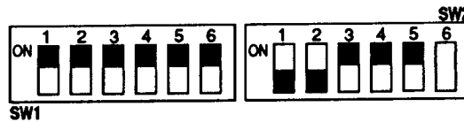
Figure 15: Factory Address Switch Settings
