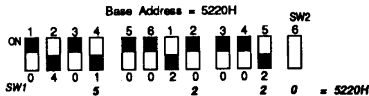
Figure 16: Address Switch Selection Examples
