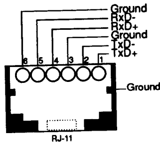
Figure 21: Output Connectors
